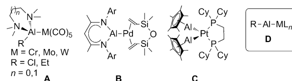
Figure 1. Transition-metal complexes of Lewis-base-coordinated ( A–C ) and Lewis-base-free ( D ) alumylenes. Ar = 2,6-(iPr) 2 C 6 H 3 .
